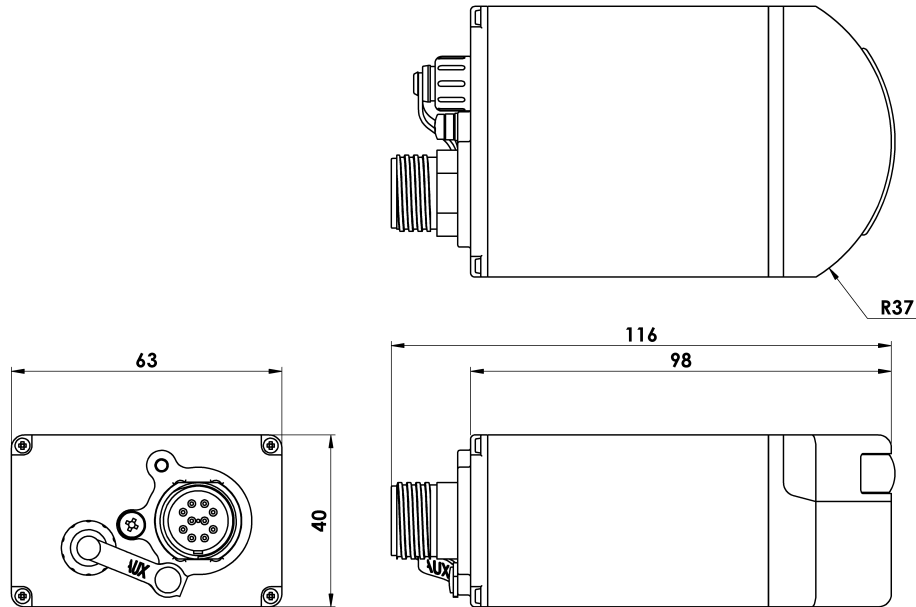
Drawing shown with Impulse MKS(W)-3L10 connector. All dimensions are in mm, not to scale.
